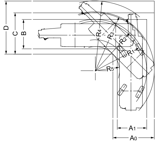
● Left turn in 4-wheel steering mode
